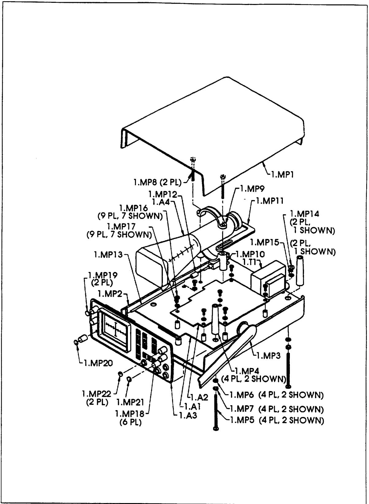
Figure 5-1. Final Assembly.
