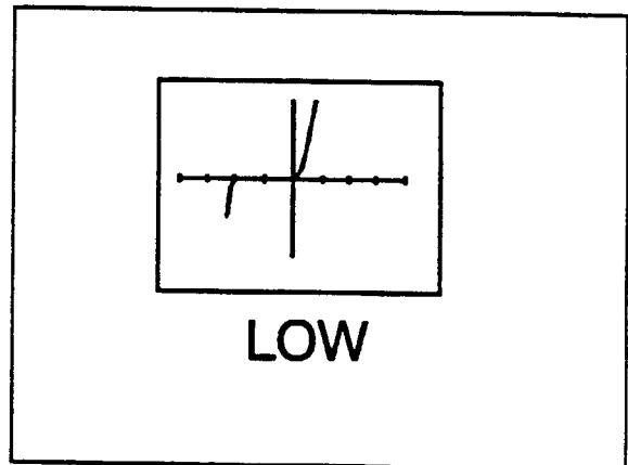
Figure 3-9b. Zener Diode Signature.
