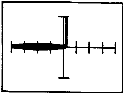
Medium 1, .1µF, 60 Hz
