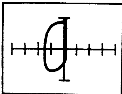
High, .1µF, 60 Hz
