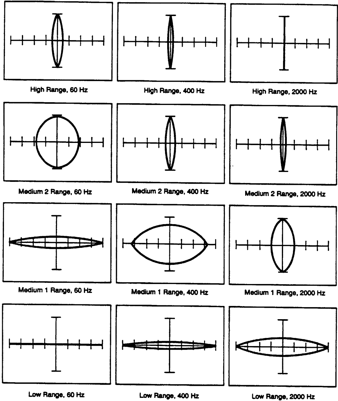
Figure 7-5. Signatures of a 0.22µF Capacitor.
