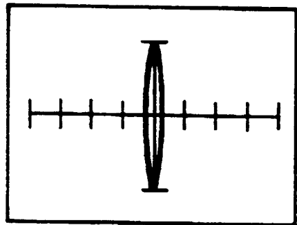
Medium 2, .1µF, 2000 Hz
