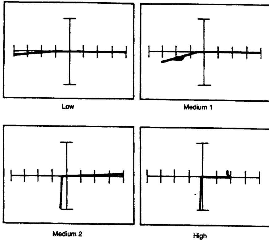
Figure 12-62. Signatures Between the CS Pin and the V_{ee} Pin of a 2708JL at 60 Hz.
