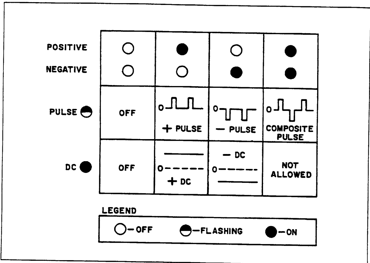
Figure 2-7. Pulse Generator Selector Chart.
