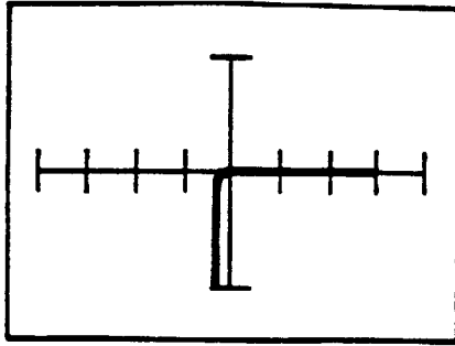
Figure 8-13. Signature with D2 or D4 Shorted in Low Range at 60 Hz.
