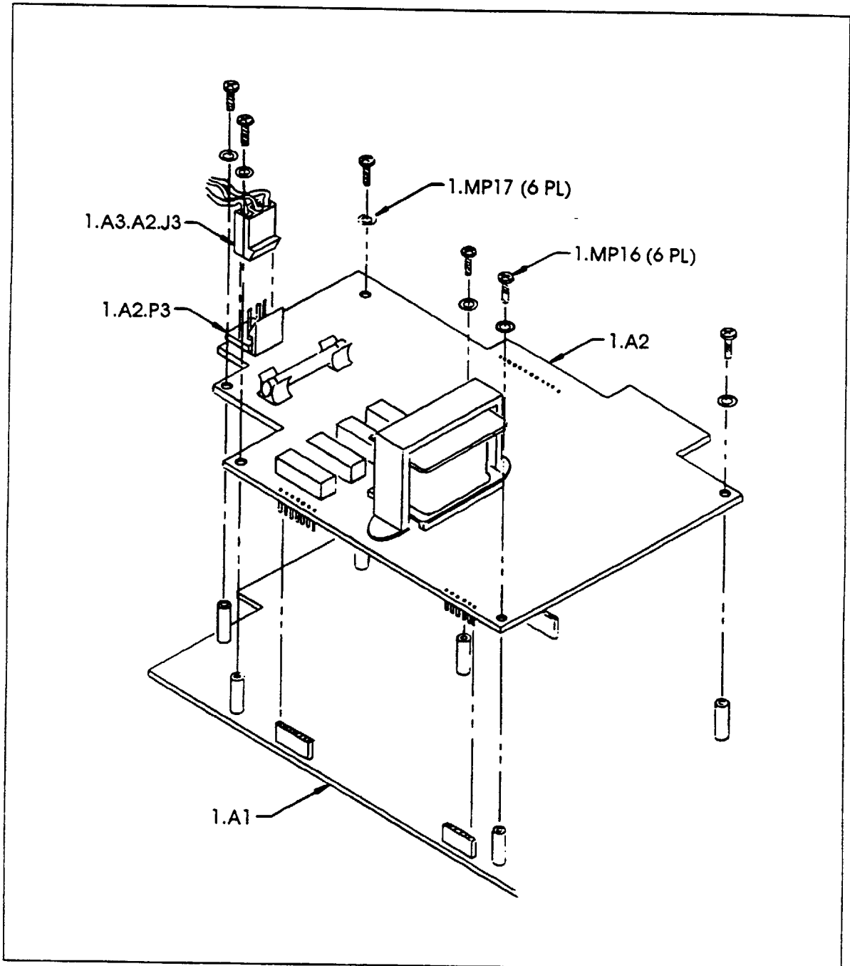
Figure 4-3. Signal PCB Assembly Removal.
