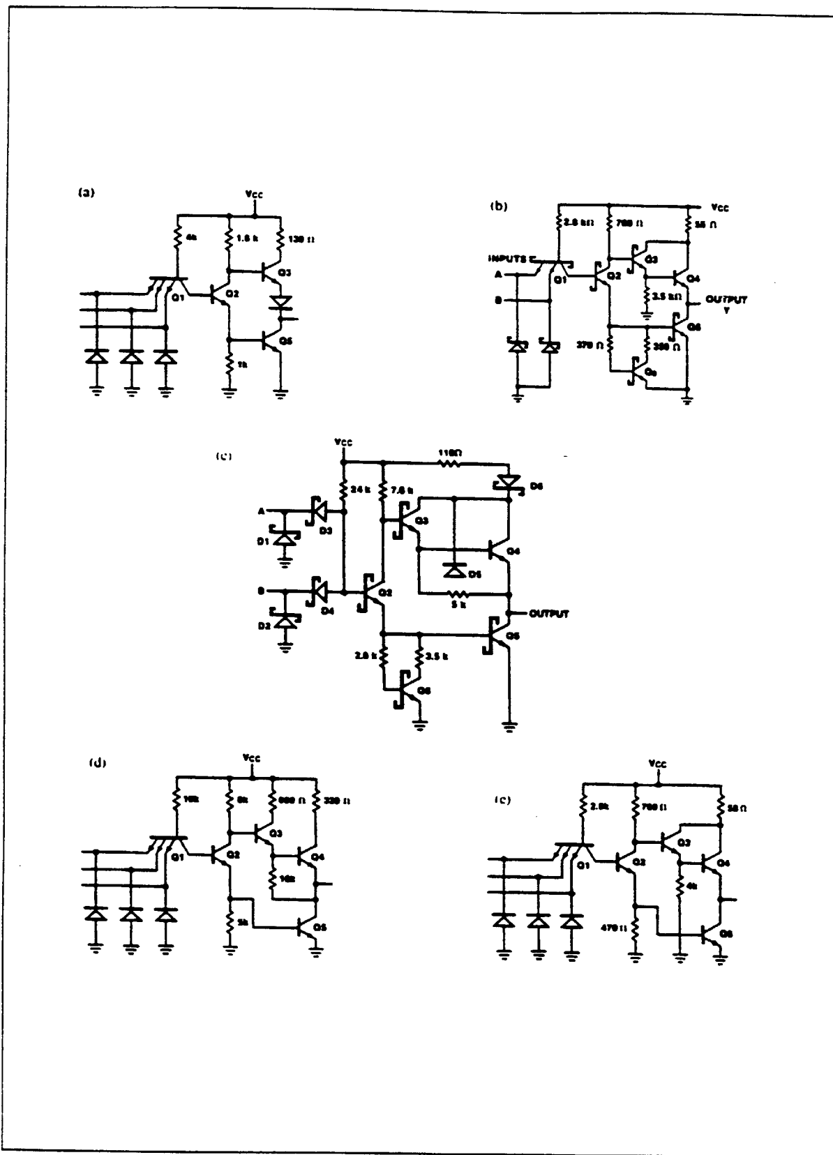
Figure 12-31. Various TTL implementations.
