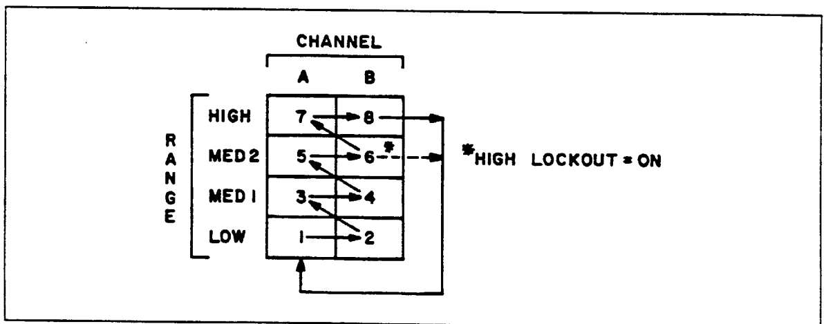
Figure 2-5. Auto/Alternate Sequence.
