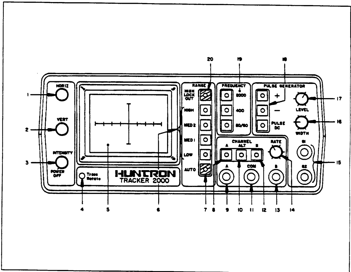
Figure 2-1. Front Panel.
